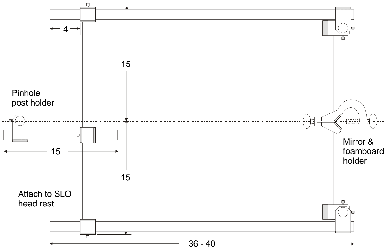
SLO Raster Calibration Attachment GT Timberlake 8/9/05 TOP VIEW
